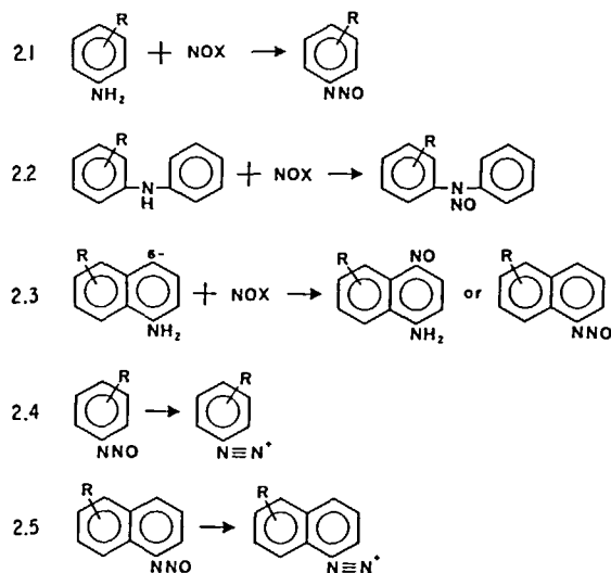
FIGURE 2. Second step nitrosation and diazonium salt formation. R: ring substituents, -\text{SO}_3\text{H} , -\text{SO}_2\text{NH}_2 , -\text{Cl} , -\text{COOH} , -\text{NO}_2 , etc. X: Cl, Br, \text{NO}_3 , .
