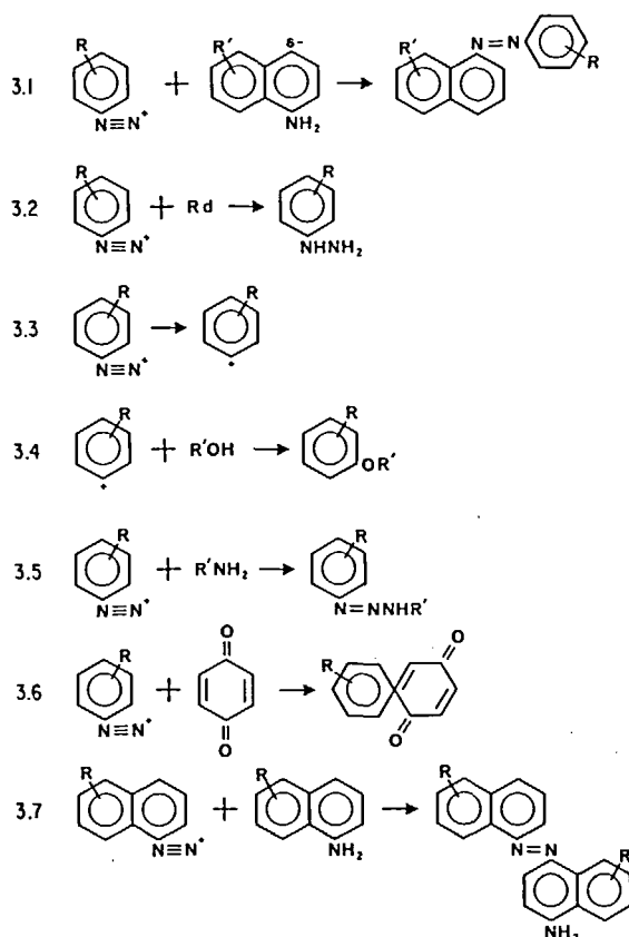
FIGURE 3. Fourth step diazotization and coupling reactions. R: ring substituents, -SO 3 H, -SO 2 NH 2 , -Cl, -COOH, -NO 2 , etc. X: Cl, Br, NO 2 , OH 2 + .
